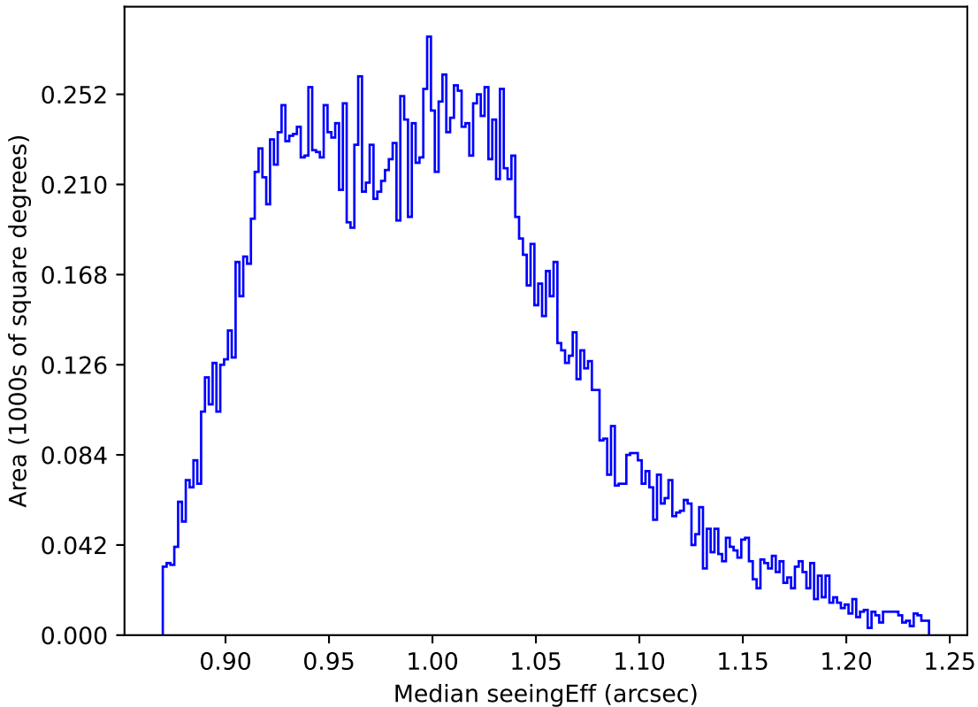
noroll_mjdp120_v3.4_10yrs All sky y band: Median seeingEff
