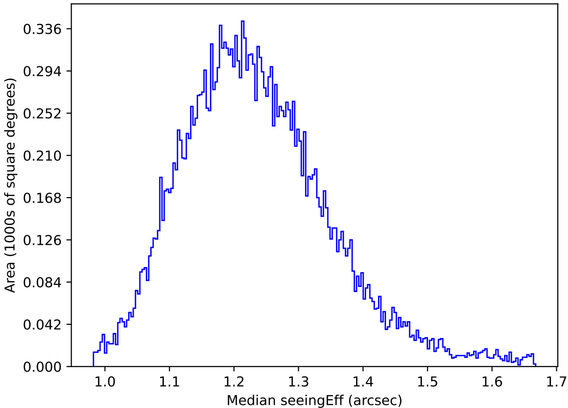
noroll_mjdp120_v3.4_10yrs All sky u band: Median seeingEff
