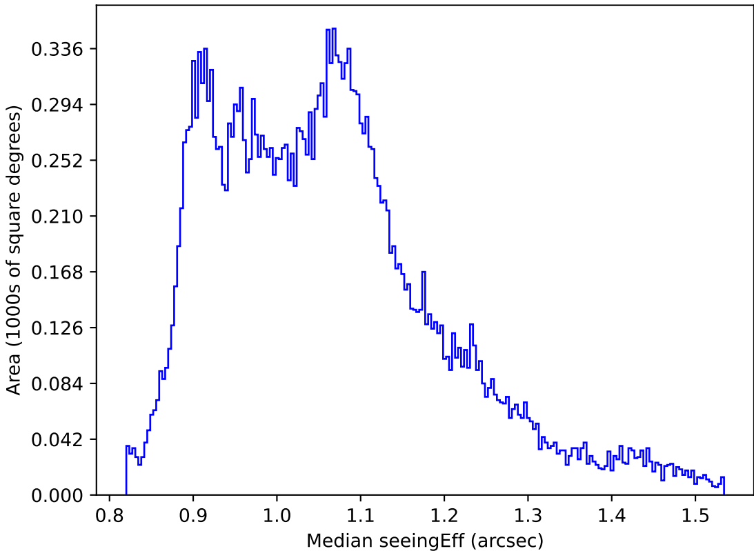
noroll_mjdp120_v3.4_10yrs All sky r band: Median seeingEff
