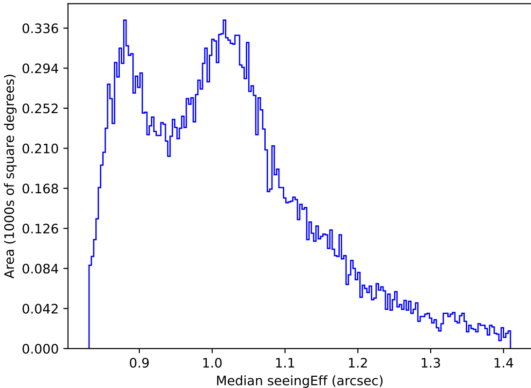
noroll_mjdp120_v3.4_10yrs All sky i band: Median seeingEff
