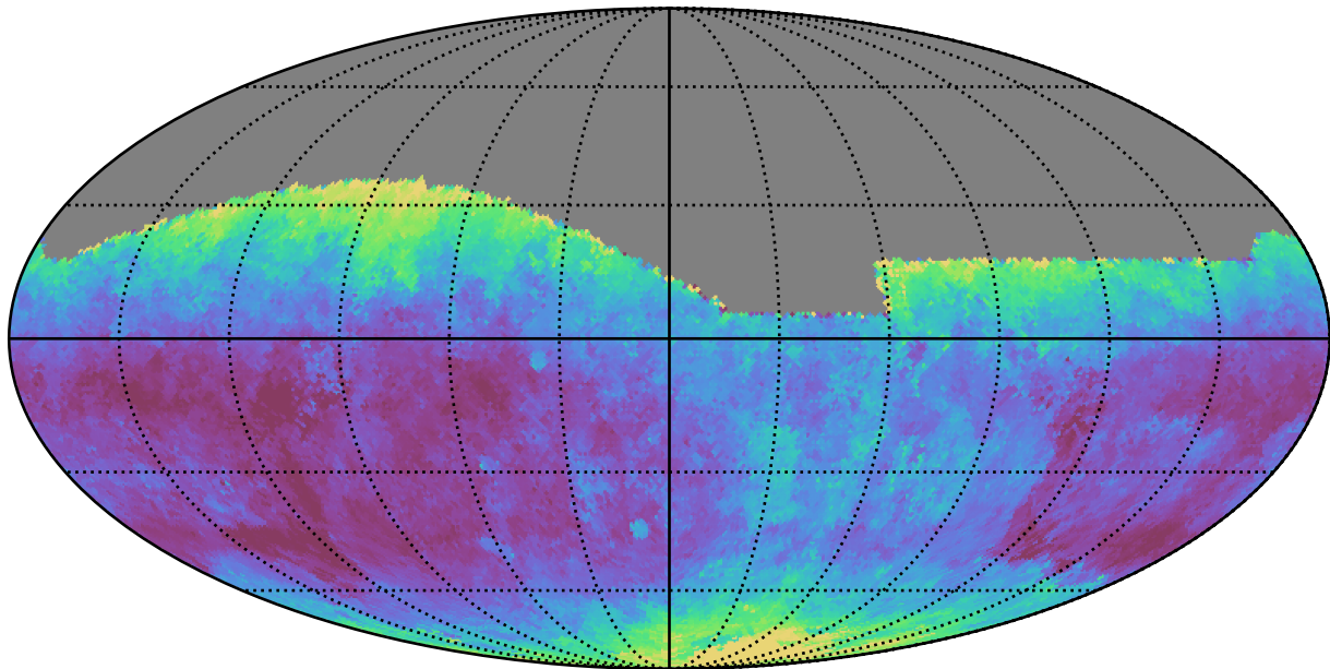
noroll_mjdp120_v3.4_10yrs All sky g band: Median seeingEff
