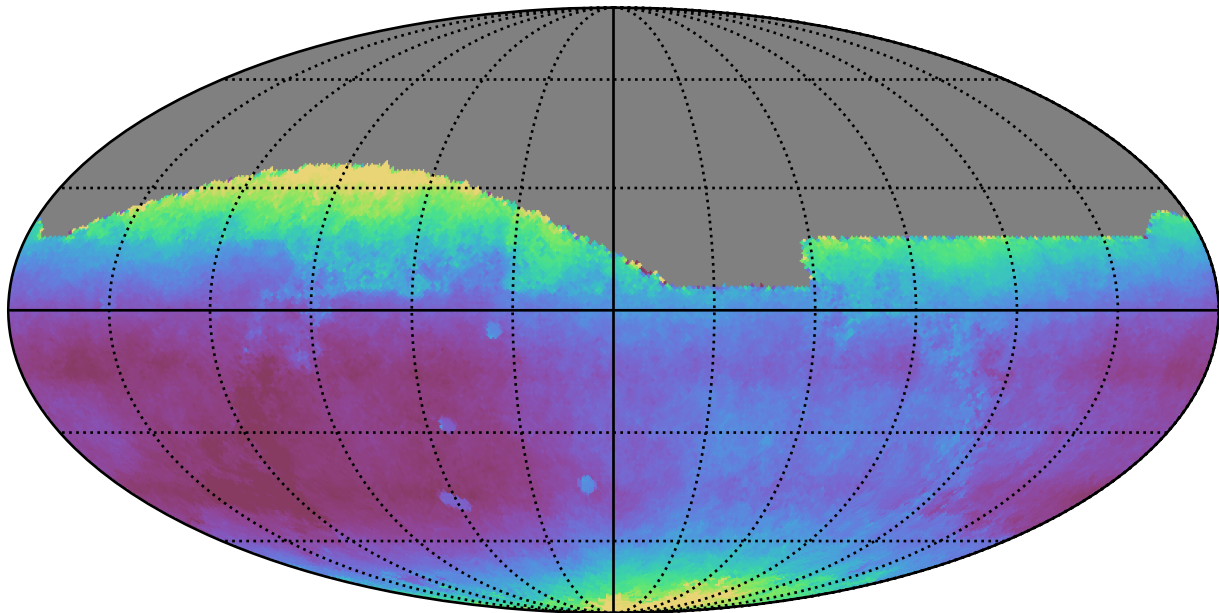
noroll_mjdp120_v3.4_10yrs All sky all bands: Median seeingEff
