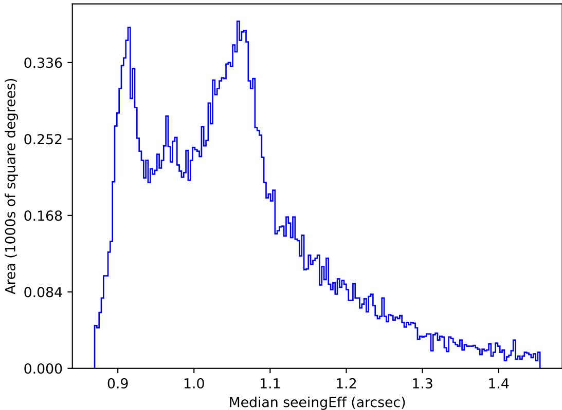
noroll_mjdp120_v3.4_10yrs All sky all bands: Median seeingEff
