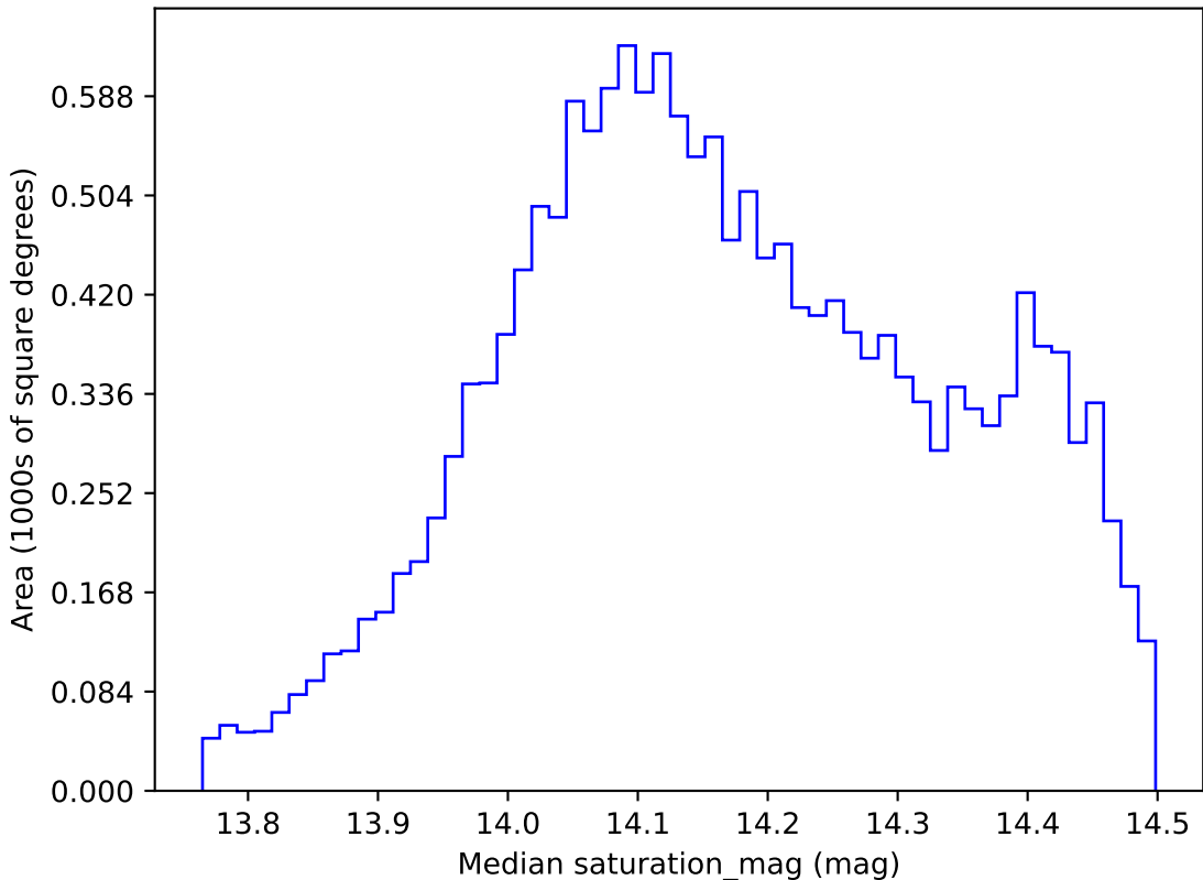
noroll_mjdp120_v3.4_10yrs WFD z band: Median saturation_mag
