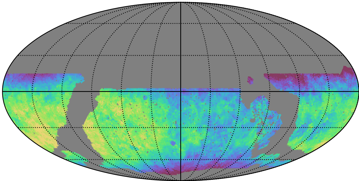
noroll_mjdp120_v3.4_10yrs WFD y band: Median saturation_mag
