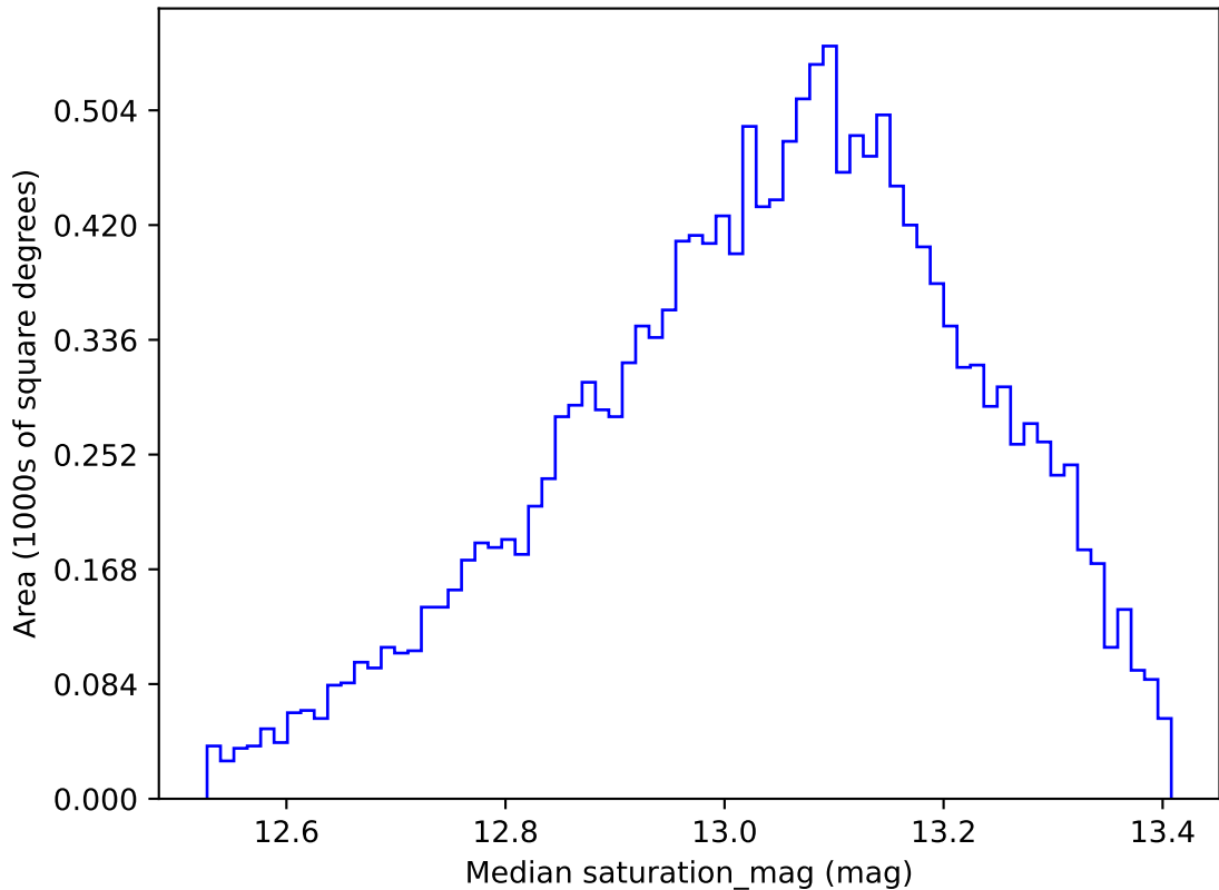
noroll_mjdp120_v3.4_10yrs WFD u band: Median saturation_mag
