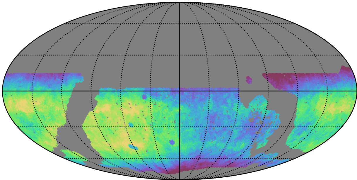
noroll_mjdp120_v3.4_10yrs WFD r band: Median saturation_mag
