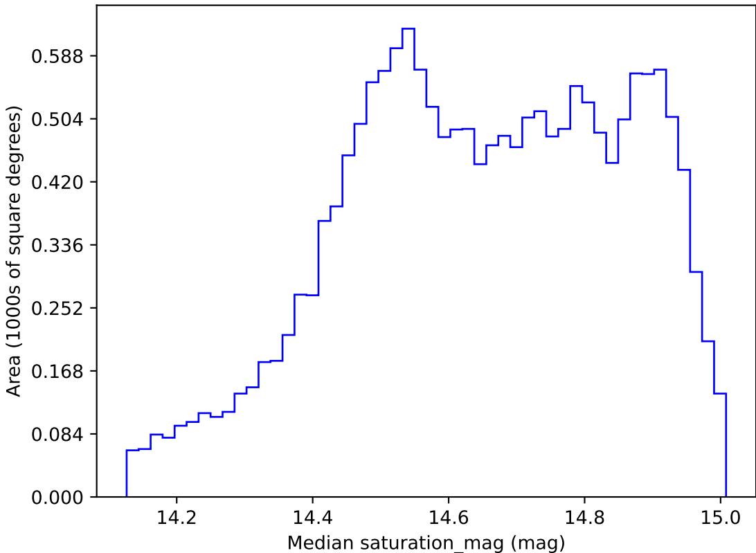
noroll_mjdp120_v3.4_10yrs WFD r band: Median saturation_mag
