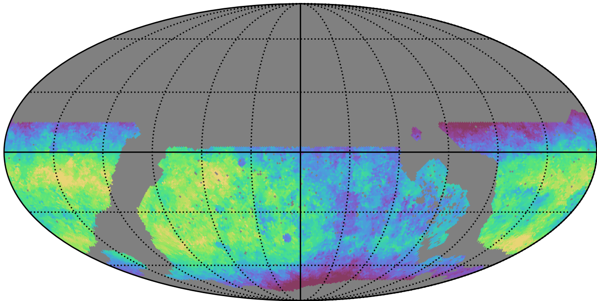
noroll_mjdp120_v3.4_10yrs WFD g band: Median saturation_mag
