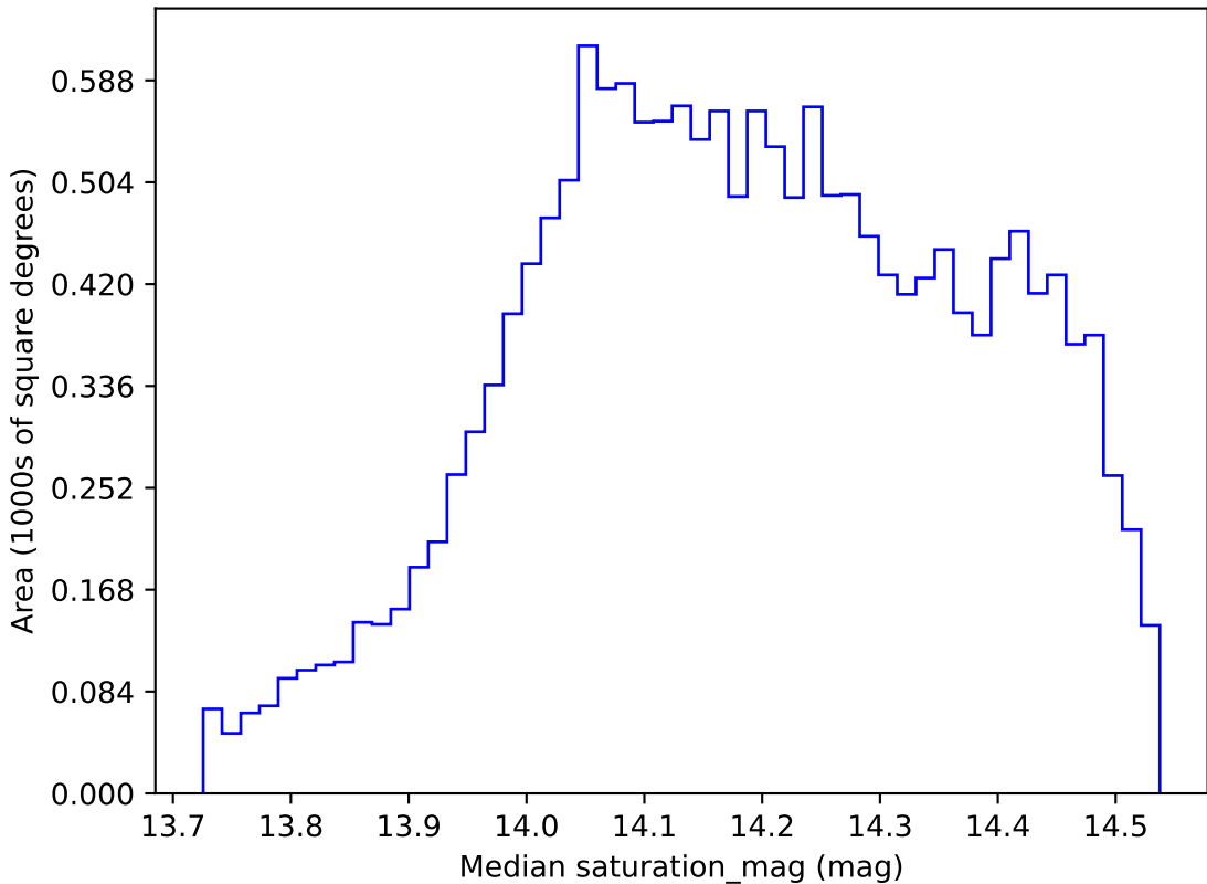
noroll_mjdp120_v3.4_10yrs WFD all bands: Median saturation_mag
