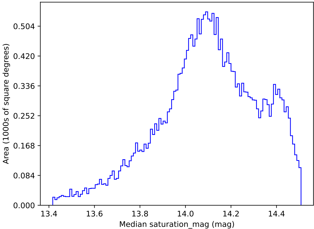
noroll_mjdp120_v3.4_10yrs All sky z band: Median saturation_mag
