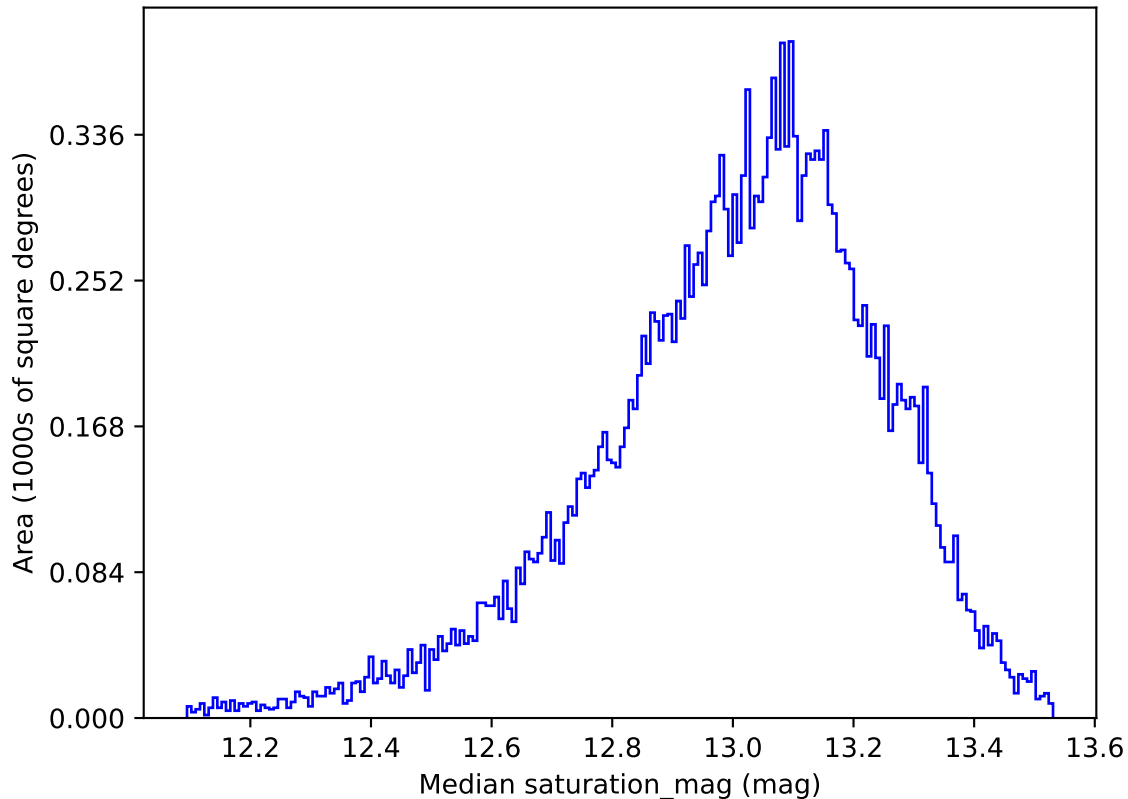
noroll_mjdp120_v3.4_10yrs All sky u band: Median saturation_mag
