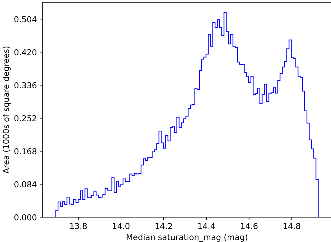
noroll_mjdp120_v3.4_10yrs All sky i band: Median saturation_mag
