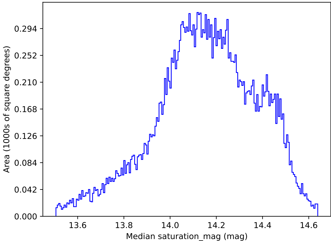
noroll_mjdp120_v3.4_10yrs All sky all bands: Median saturation_mag
