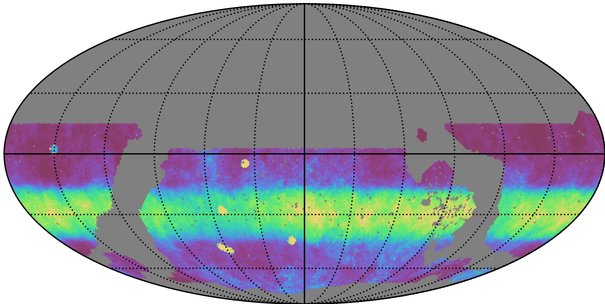
noroll_mjdp120_v3.4_10yrs WFD z band: Median normairmass
