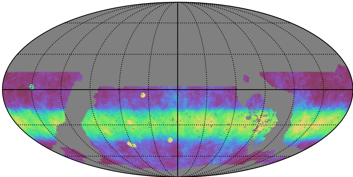
noroll_mjdp120_v3.4_10yrs WFD y band: Median normairmass
