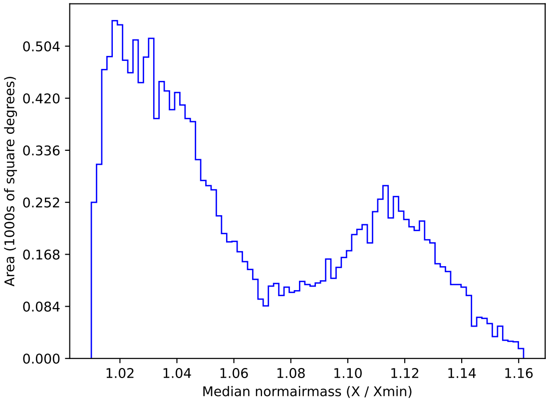
noroll_mjdp120_v3.4_10yrs WFD u band: Median normairmass
