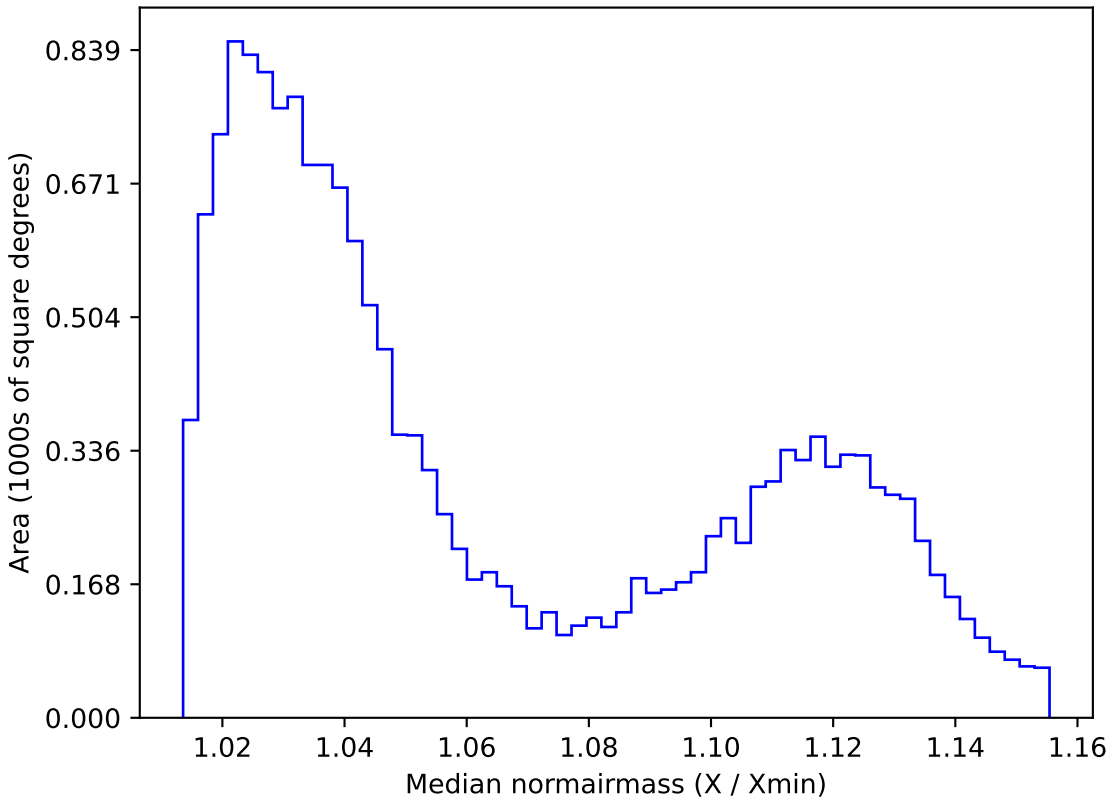
noroll_mjdp120_v3.4_10yrs WFD r band: Median normairmass
