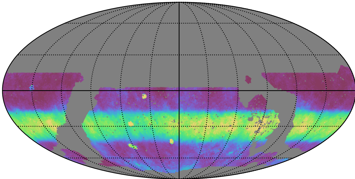
noroll_mjdp120_v3.4_10yrs WFD i band: Median normairmass
