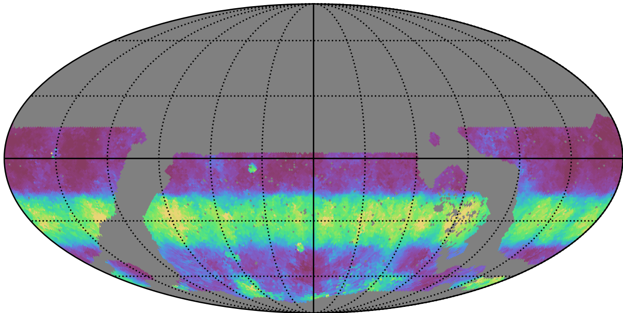
noroll_mjdp120_v3.4_10yrs WFD g band: Median normairmass
