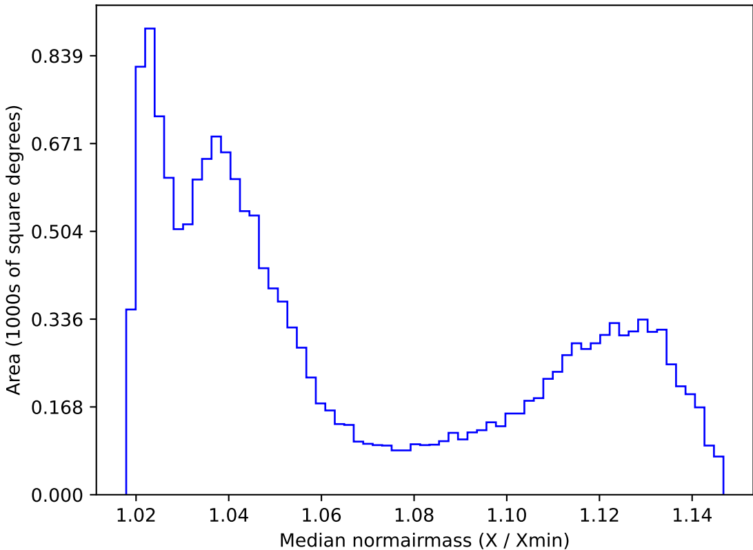
noroll_mjdp120_v3.4_10yrs WFD all bands: Median normairmass
