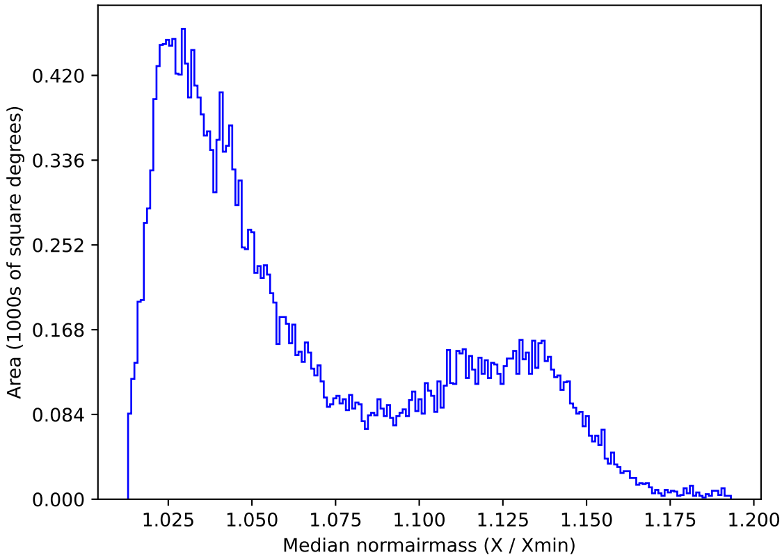
noroll_mjdp120_v3.4_10yrs All sky z band: Median normairmass
