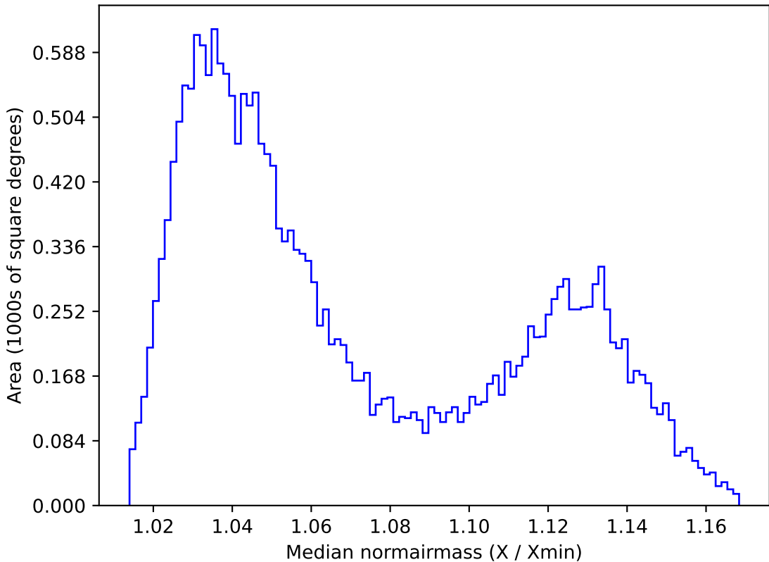
noroll_mjdp120_v3.4_10yrs All sky y band: Median normairmass
