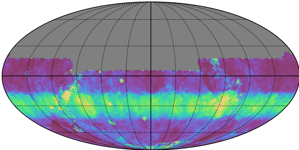
noroll_mjdp120_v3.4_10yrs All sky u band: Median normairmass
