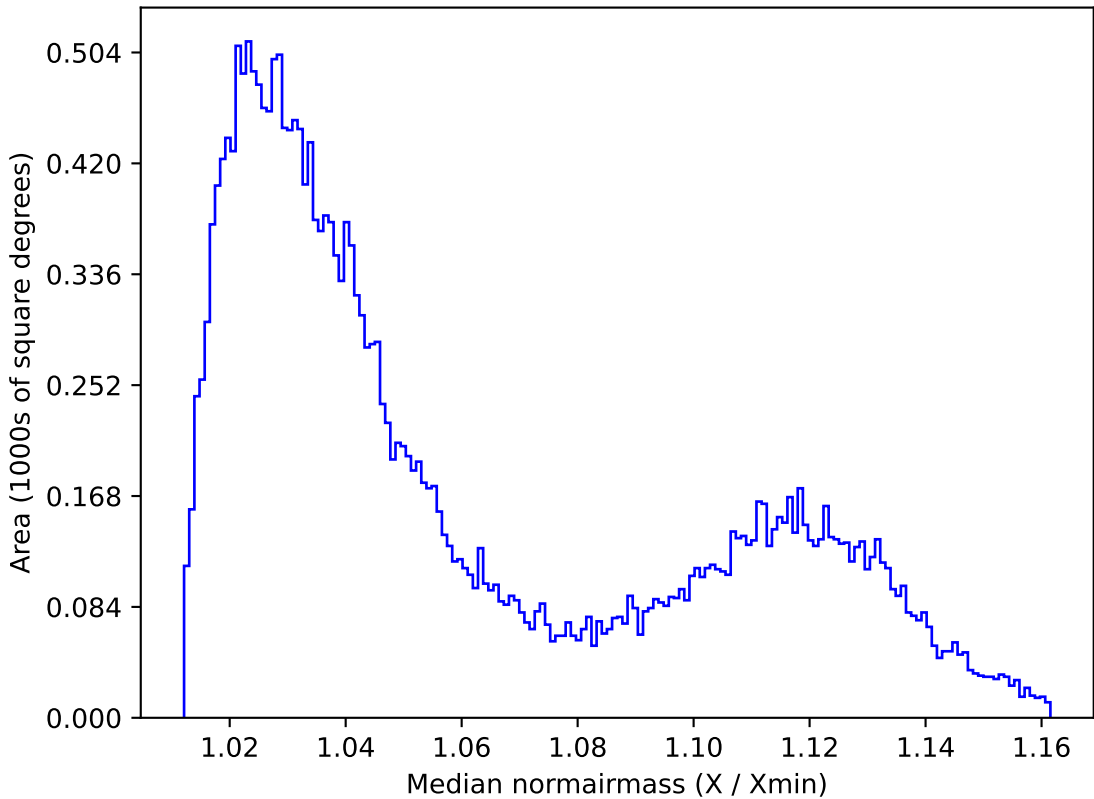
noroll_mjdp120_v3.4_10yrs All sky r band: Median normairmass
