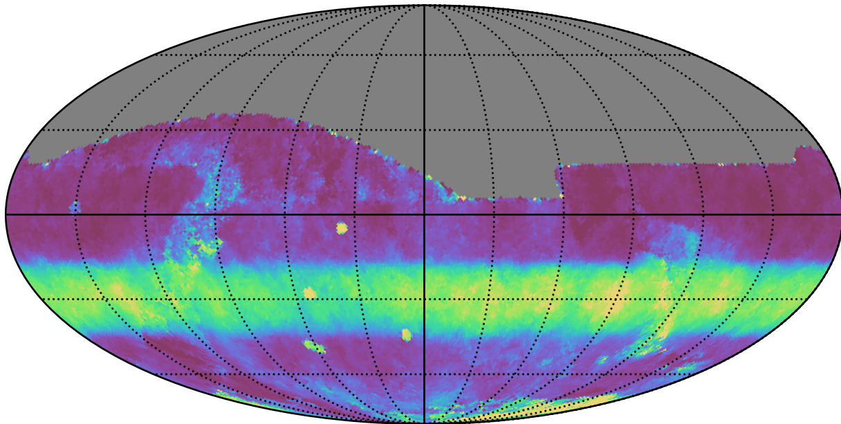
noroll_mjdp120_v3.4_10yrs All sky i band: Median normairmass
