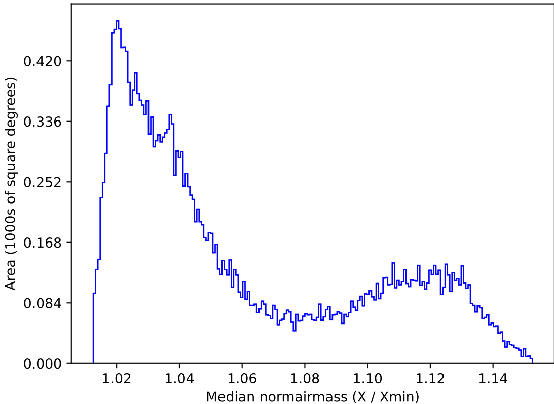
noroll_mjdp120_v3.4_10yrs All sky i band: Median normairmass
