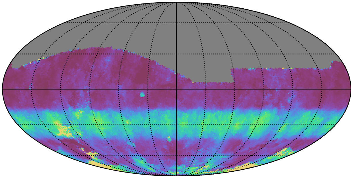
noroll_mjdp120_v3.4_10yrs All sky g band: Median normairmass
