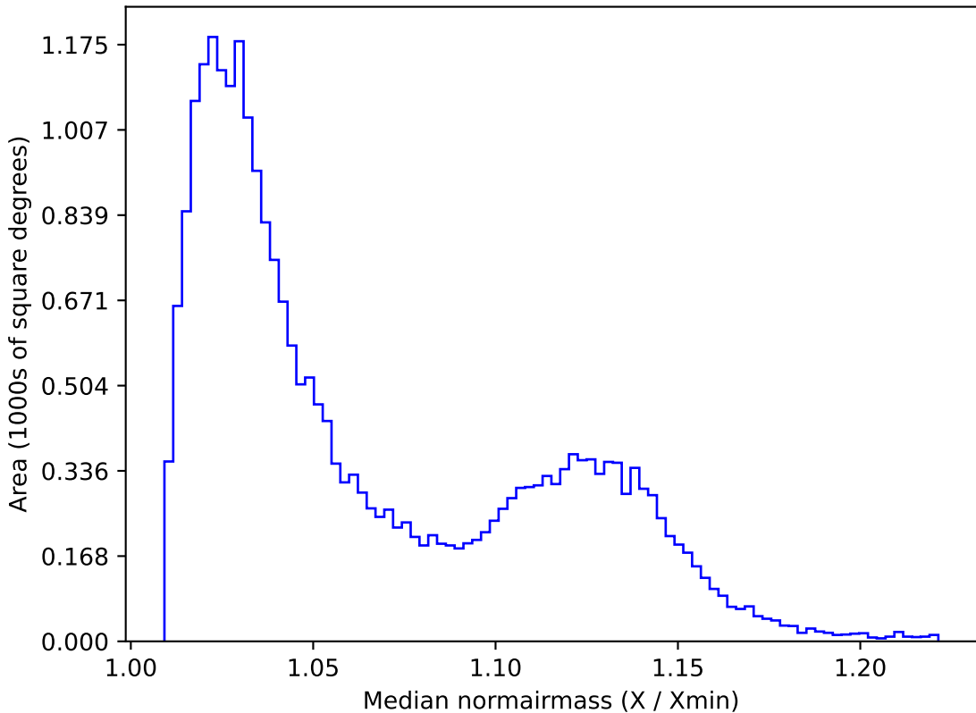
noroll_mjdp120_v3.4_10yrs All sky g band: Median normairmass
