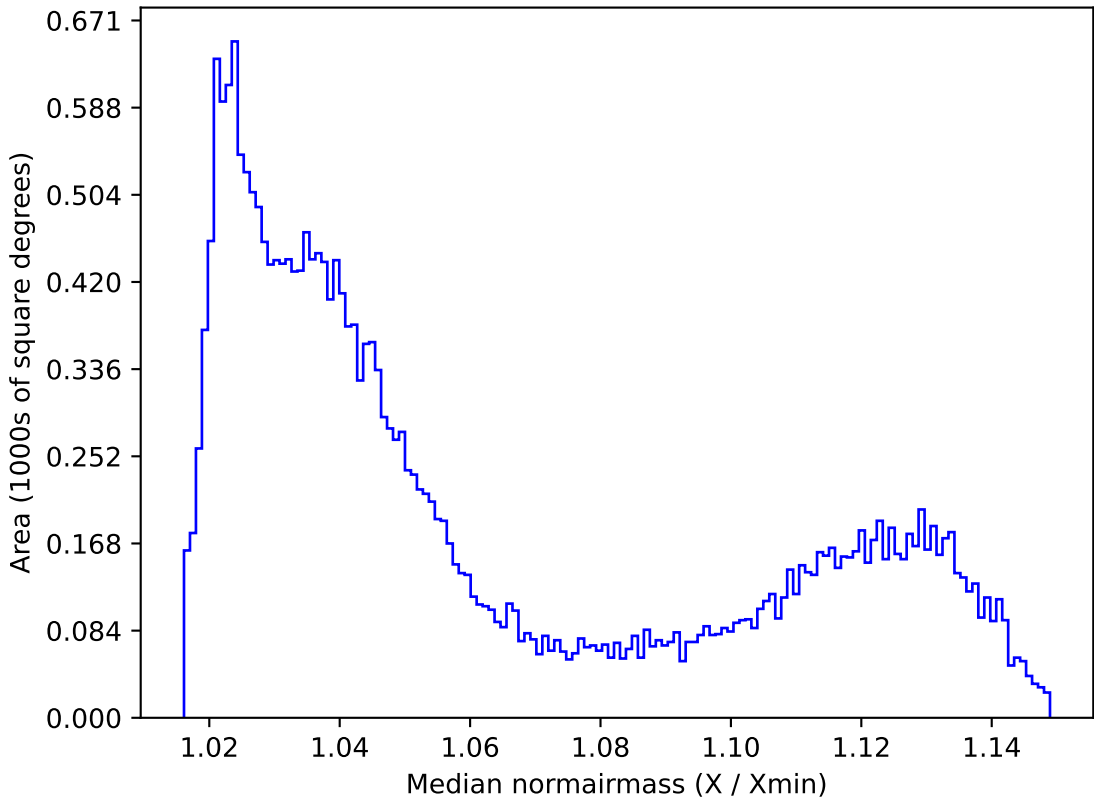
noroll_mjdp120_v3.4_10yrs All sky all bands: Median normairmass
