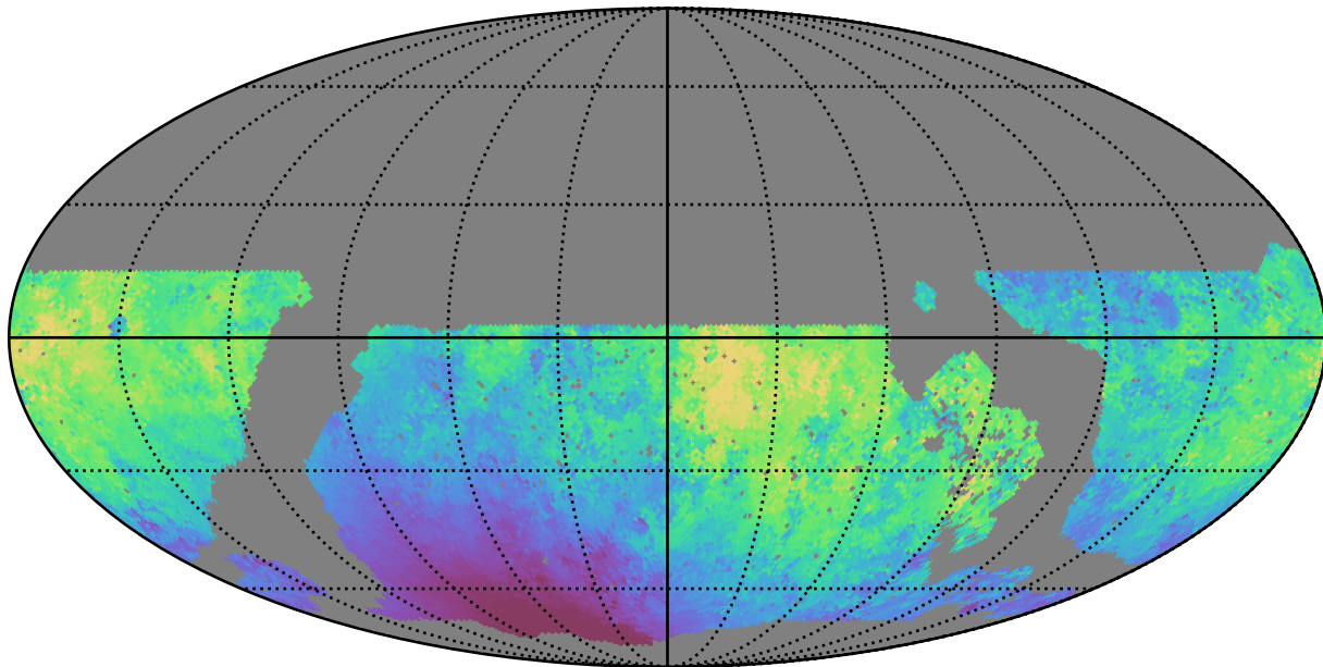
noroll_mjdp120_v3.4_10yrs WFD u band: Median moonDistance
