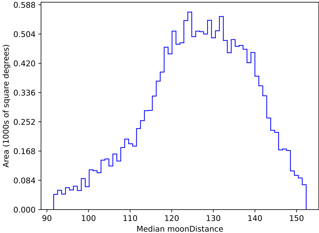
noroll_mjdp120_v3.4_10yrs WFD u band: Median moonDistance
