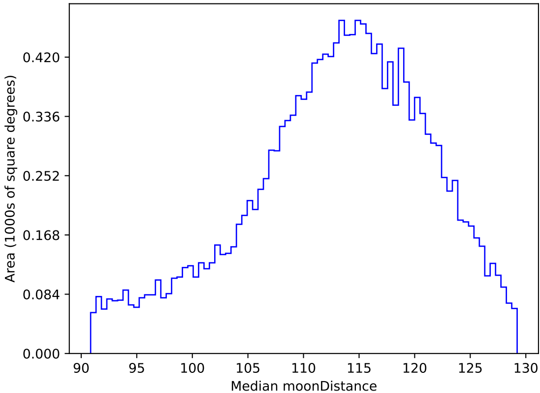
noroll_mjdp120_v3.4_10yrs WFD r band: Median moonDistance
