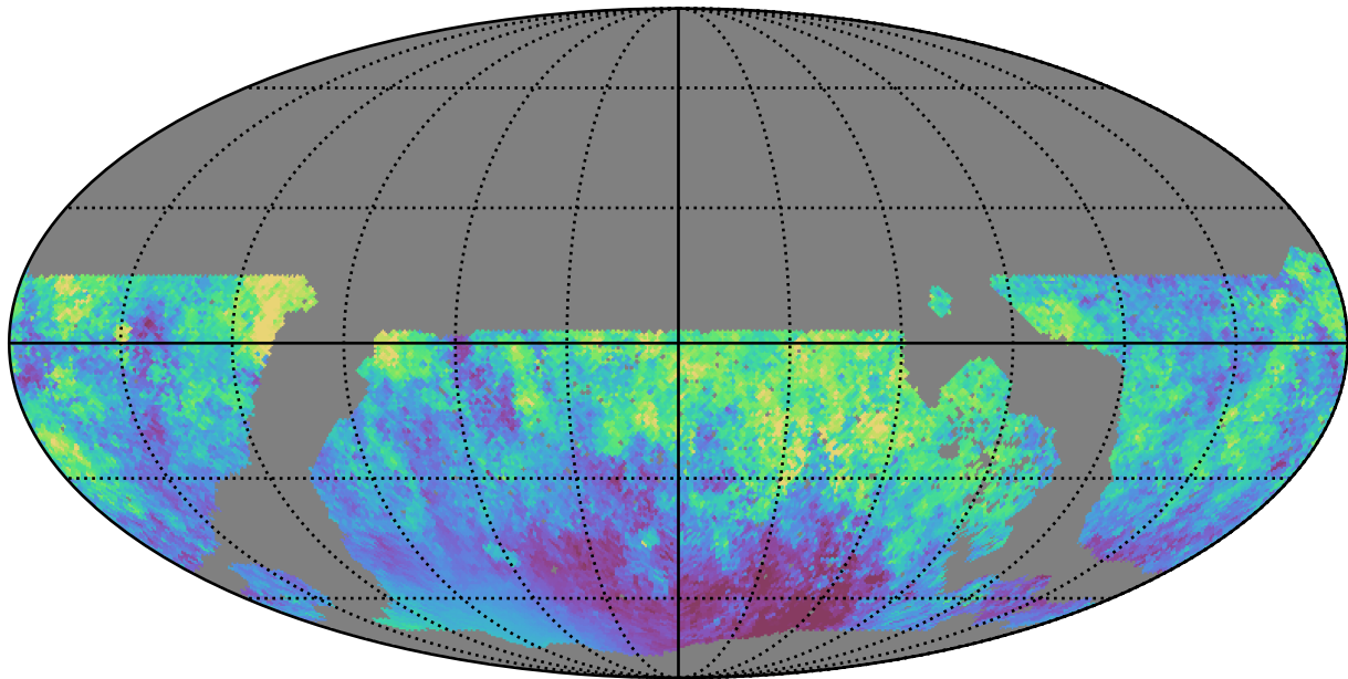
noroll_mjdp120_v3.4_10yrs WFD i band: Median moonDistance
