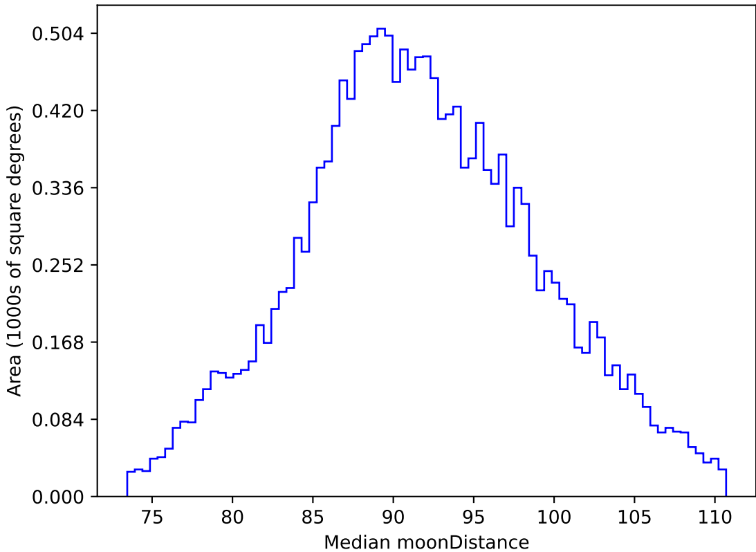
noroll_mjdp120_v3.4_10yrs WFD i band: Median moonDistance
