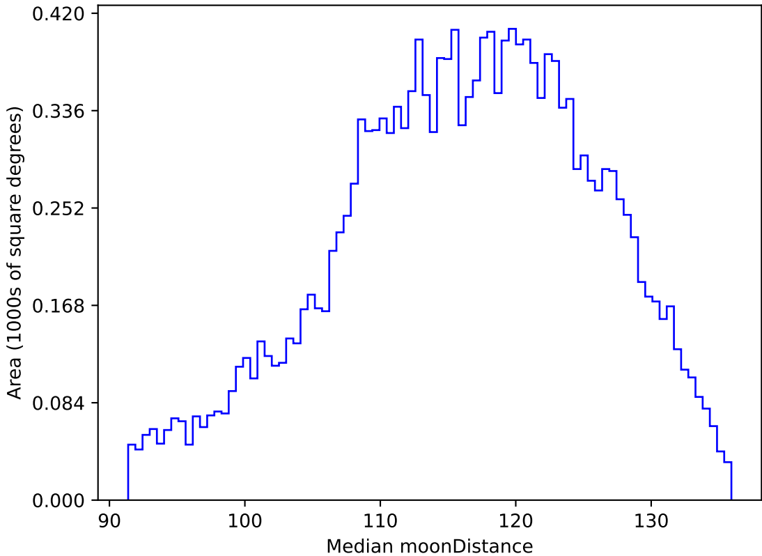
noroll_mjdp120_v3.4_10yrs WFD g band: Median moonDistance
