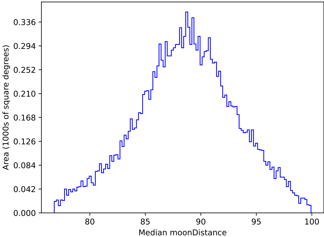
noroll_mjdp120_v3.4_10yrs WFD all bands: Median moonDistance
