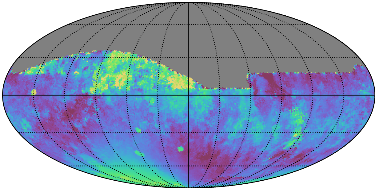
noroll_mjdp120_v3.4_10yrs All sky z band: Median moonDistance
