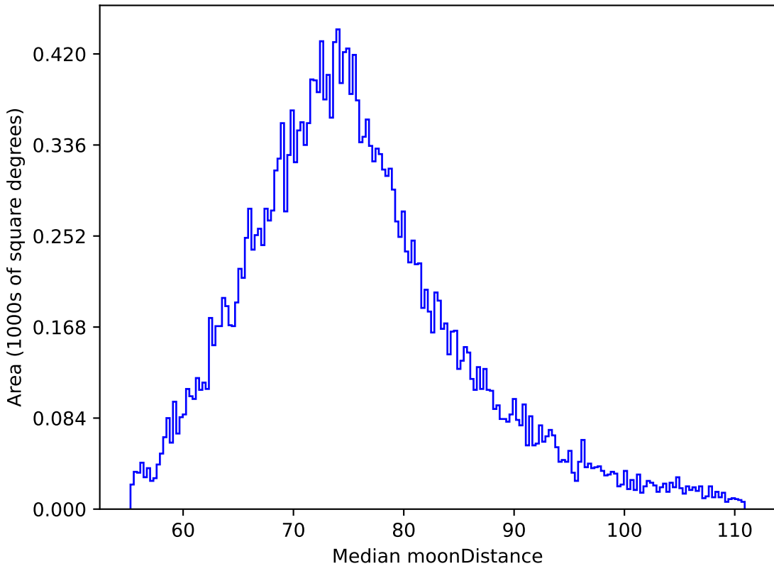
noroll_mjdp120_v3.4_10yrs All sky z band: Median moonDistance
