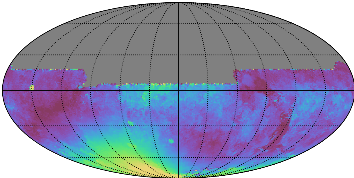
noroll_mjdp120_v3.4_10yrs All sky y band: Median moonDistance
