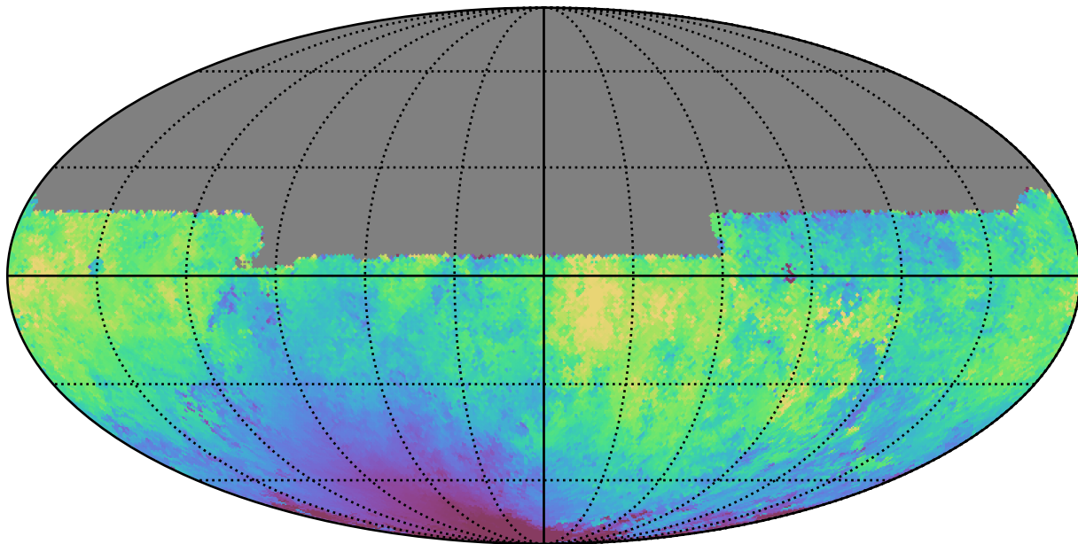
noroll_mjdp120_v3.4_10yrs All sky u band: Median moonDistance
