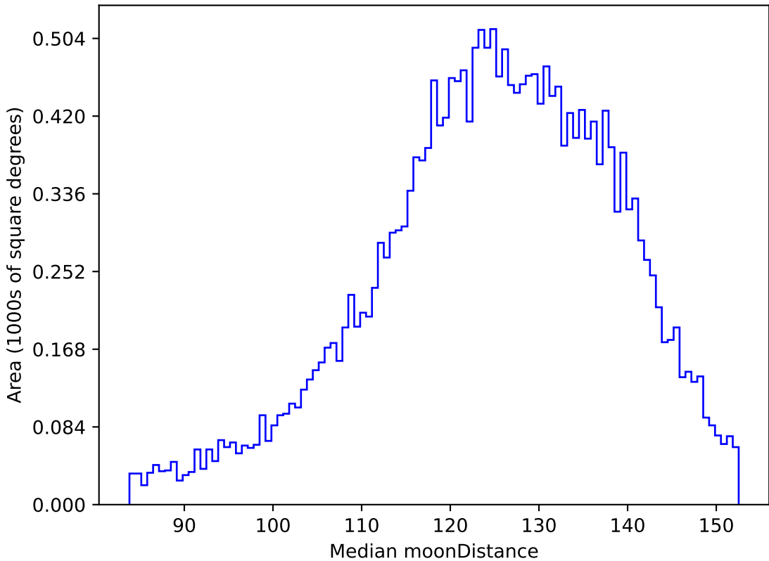
noroll_mjdp120_v3.4_10yrs All sky u band: Median moonDistance
