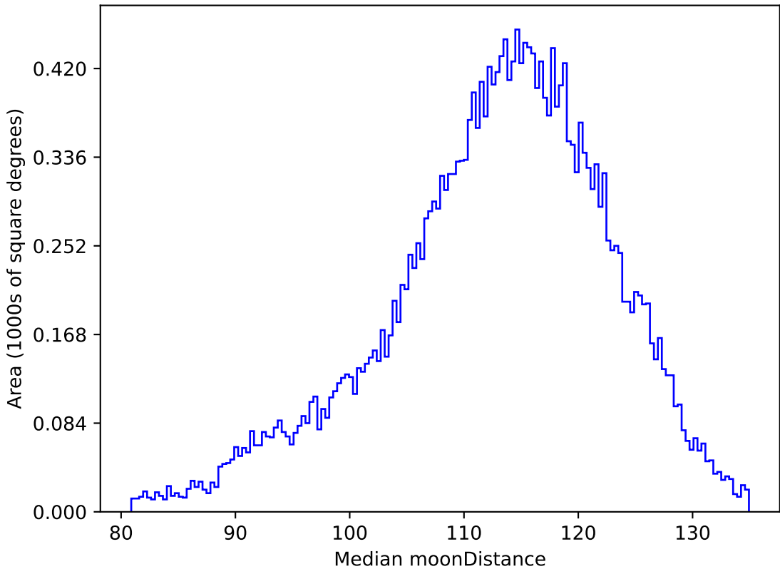
noroll_mjdp120_v3.4_10yrs All sky r band: Median moonDistance
