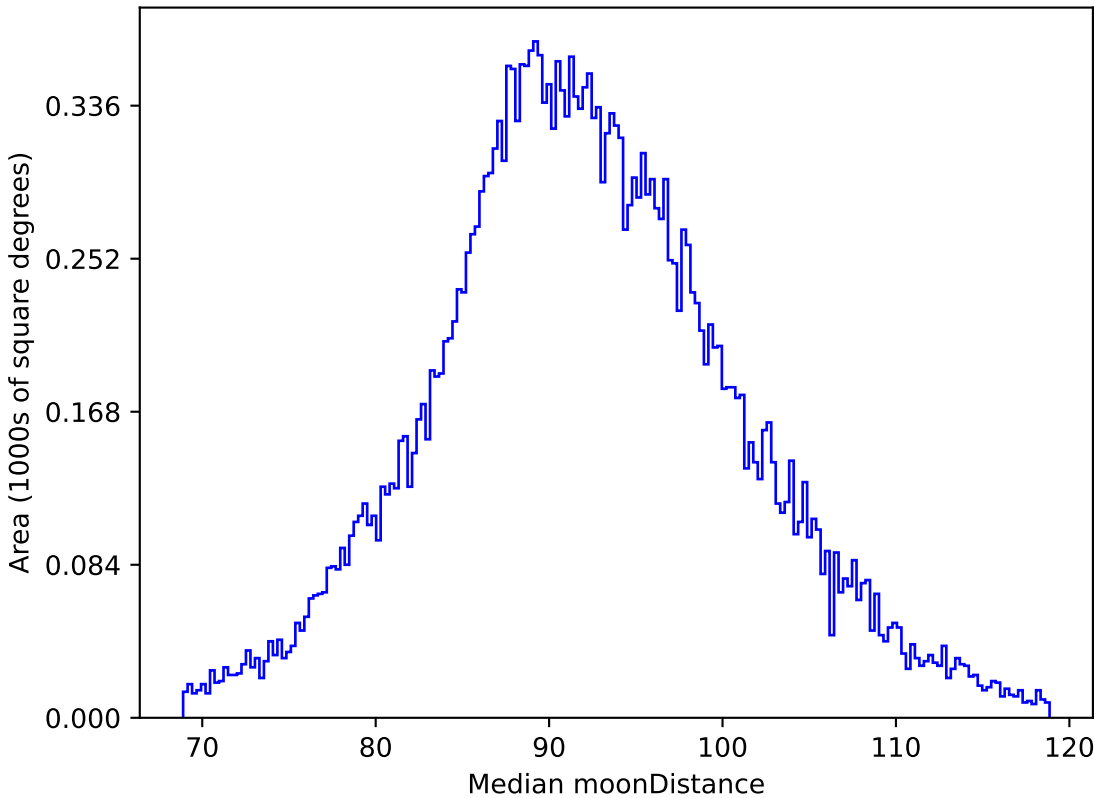
noroll_mjdp120_v3.4_10yrs All sky i band: Median moonDistance
