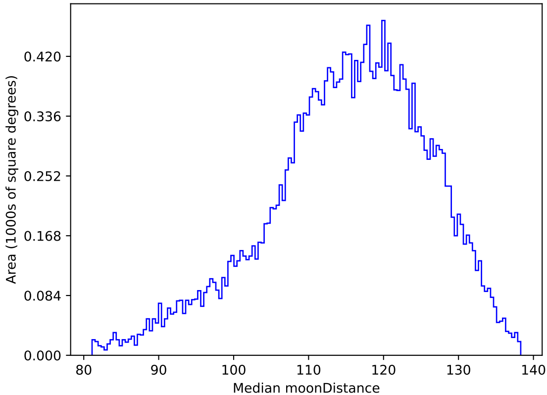
noroll_mjdp120_v3.4_10yrs All sky g band: Median moonDistance
