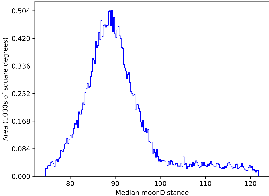
noroll_mjdp120_v3.4_10yrs All sky all bands: Median moonDistance
